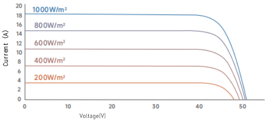
I-P/P-V Curve at Different Irradiation (710W)
