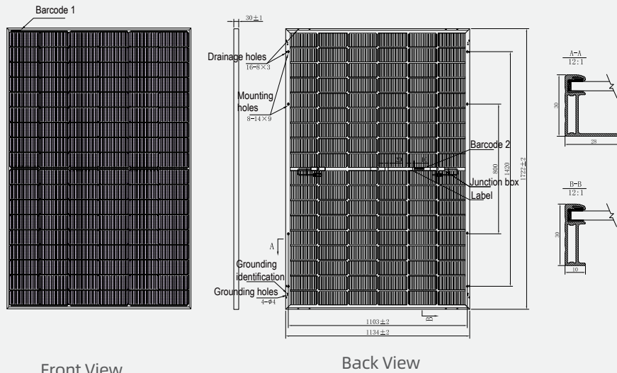
DIMENSIONS OF PV MODULE(mm)
